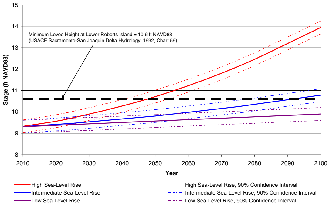
Figure 15 - Burns Cutoff Gage Station Estimated Stage with 1/50 Annual Exceedance Probability, 2010 through 2100
